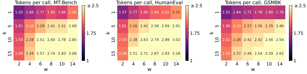
Figure 9: Tokens per call across datasets for Vicuna13B for varied (k, w) .
