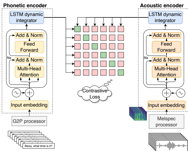
Figure 1. SCRAPS model architecture, with a phonetic encoder in the left hand side, and an acoustic encoder in the right hand side.
