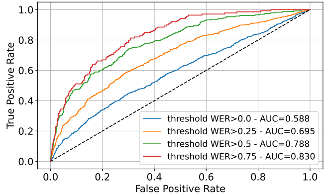
Figure 5. ROC of h-WER>T classification using SCRAPS(VC, source) scores for different thresholds T.
