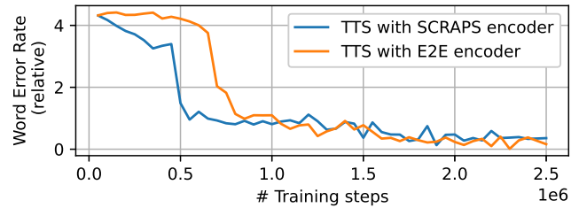
Figure 4. Word Error Rate (WER) of the TTS models, relative to the WER over the test set recordings. The two lines represent how the intelligibility of the model improves as the model trains for the architectures with pretrained SCRAPS and with E2E phonetic encoder. The WER has been measured with a pretrained ASR model over a set of 512 sentences unseen during training, synthesized every 25,000 training steps. The WER represented in the figure is relative to the recordings WER.
