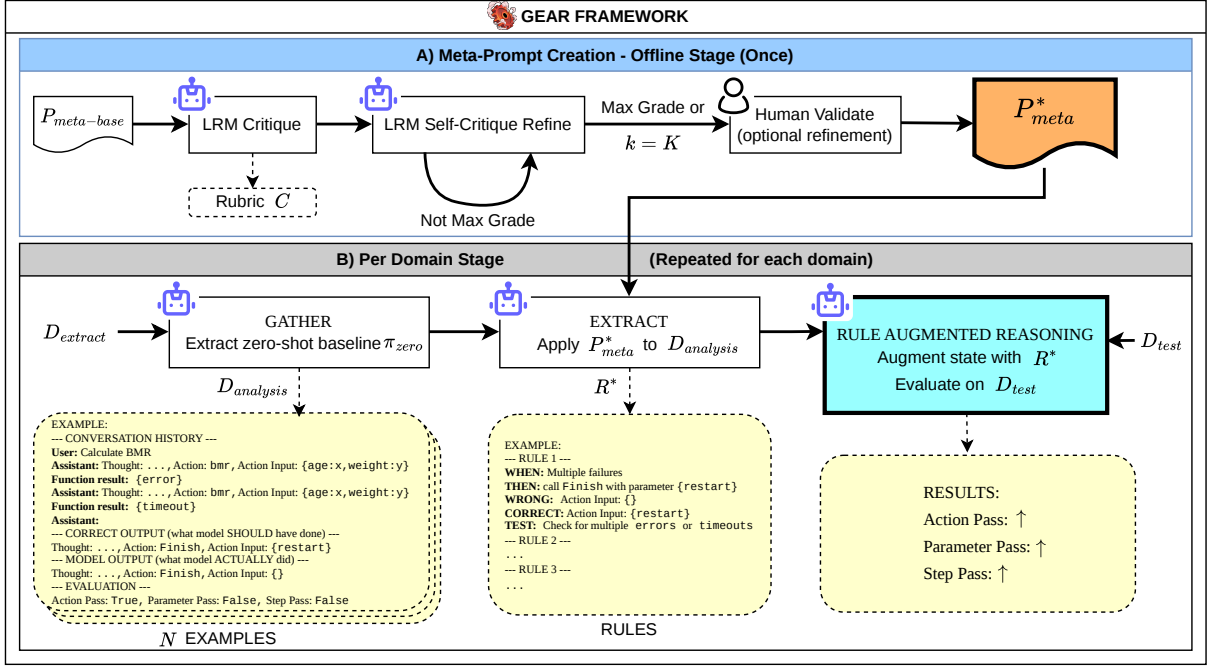
Figure 2: GEAR framework overview. The offline stage creates a domain-agnostic meta-prompt P_{meta}^* through iterative LRM self-critique with optional human validation. The per-domain stage executes three phases: Gather (collect baseline predictions), Extract (synthesize rules via meta-reasoning), and Rule-Augmented Reasoning (evaluate with rule-augmented state). The meta-prompt is created once and reused across all domains.
