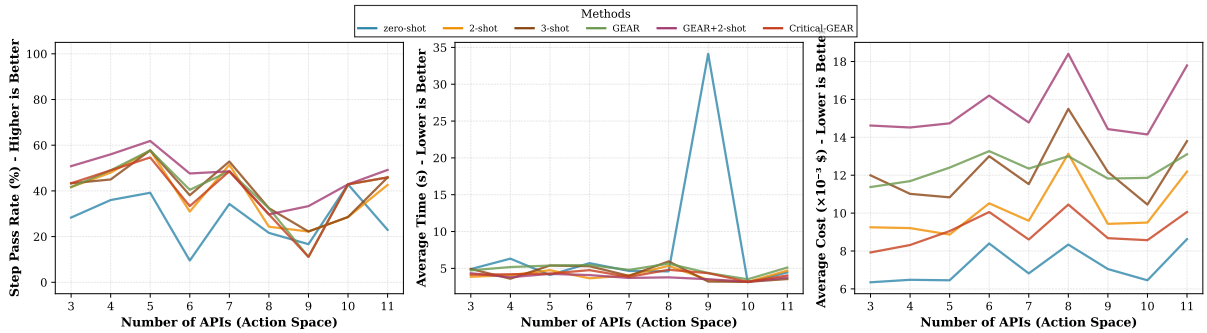
Figure 22: Performance, latency, and cost as a function of action space complexity (number of APIs) on Qwen3-30B. Unlike trajectory complexity, performance does not show clear degradation with larger action spaces.
