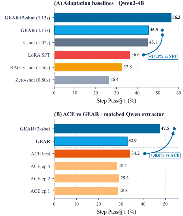
Figure 1: On Qwen3-4B, GEAR outperforms LoRA SFT (+24.3%) and RAG-3-shot (+38.5%); GEAR+2-shot nearly doubles zero-shot Step Pass@1 (A). With a matched Qwen extractor, GEAR+2-shot exceeds ACE’s best playbook by +38.8% (B).
