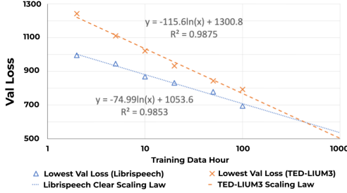
Figure 3: Comparing the scaling law between validation loss and training data size for the LibriSpeech and TED-LIUM3 training datasets.
