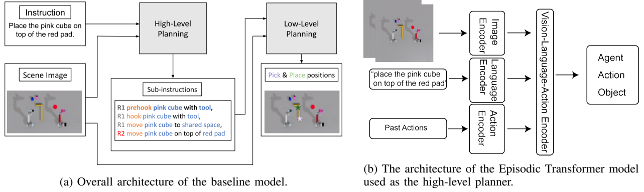
Fig. 2: Our baseline model involves a high-level task planning module and a low-level planning module. The high-level planning module takes as input the top-down fused scene image and human instruction to generate sub-instructions that assign the corresponding sub-tasks to robots based on their limitations. Each sub-task is specified by action primitives (in orange) and objects (in blue). The low-level planning module uses the sub-instruction and top-down projection of the scene to generate pick and place locations (visualized as purple and green stars respectively) of the gripper in the scene.
