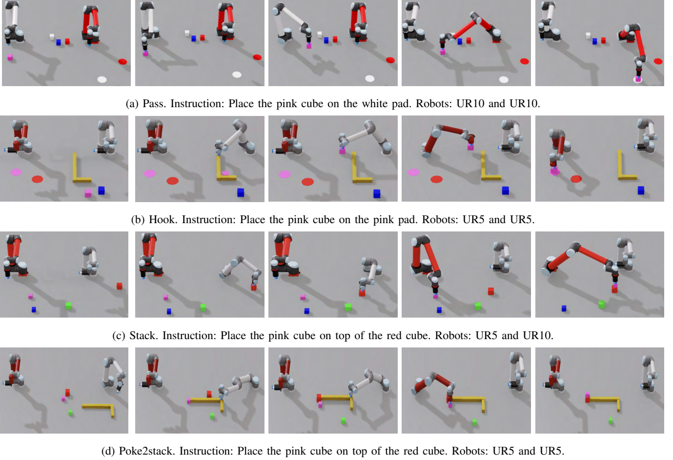
Fig. 1: Expert demonstrations and high-level instructions of tasks in LEMMA. We use minimal instructions that specify the goal, thus, it is possible that two different tasks may have the same instruction. E.g., tasks in (c) and (d) have the same instruction, but (d) requires robots to make use of the tool to poke the blocks so that the red robot can reach them. Note that the pair of robots involved in each demonstration can be different. The pair of robots in homogeneous settings (e.g., a, b, and d) have the same reach, while in heterogenous cases the reach can be different for each robot (e.g., c).
