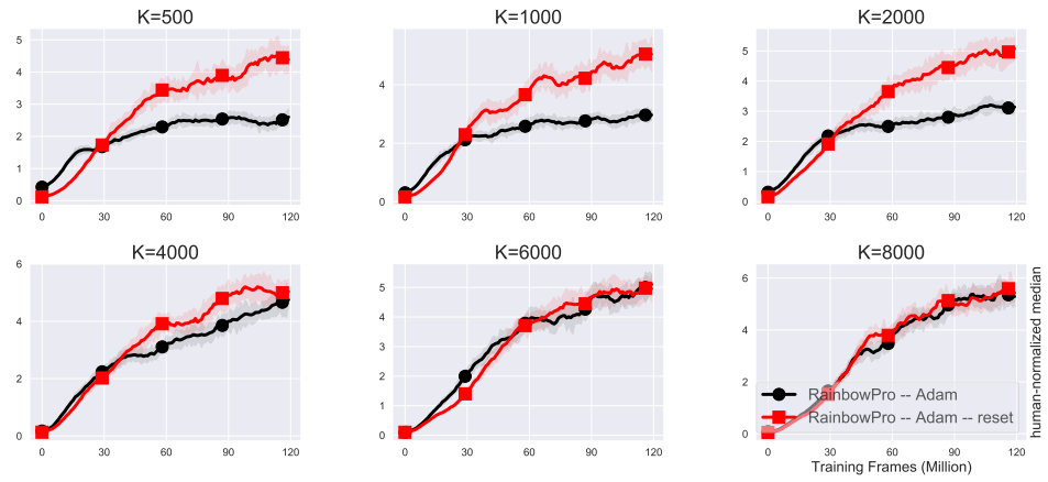
Figure 42: A comparison between Rainbow Pro with and without resetting Adam on the 12 Atari games for different values of K .
