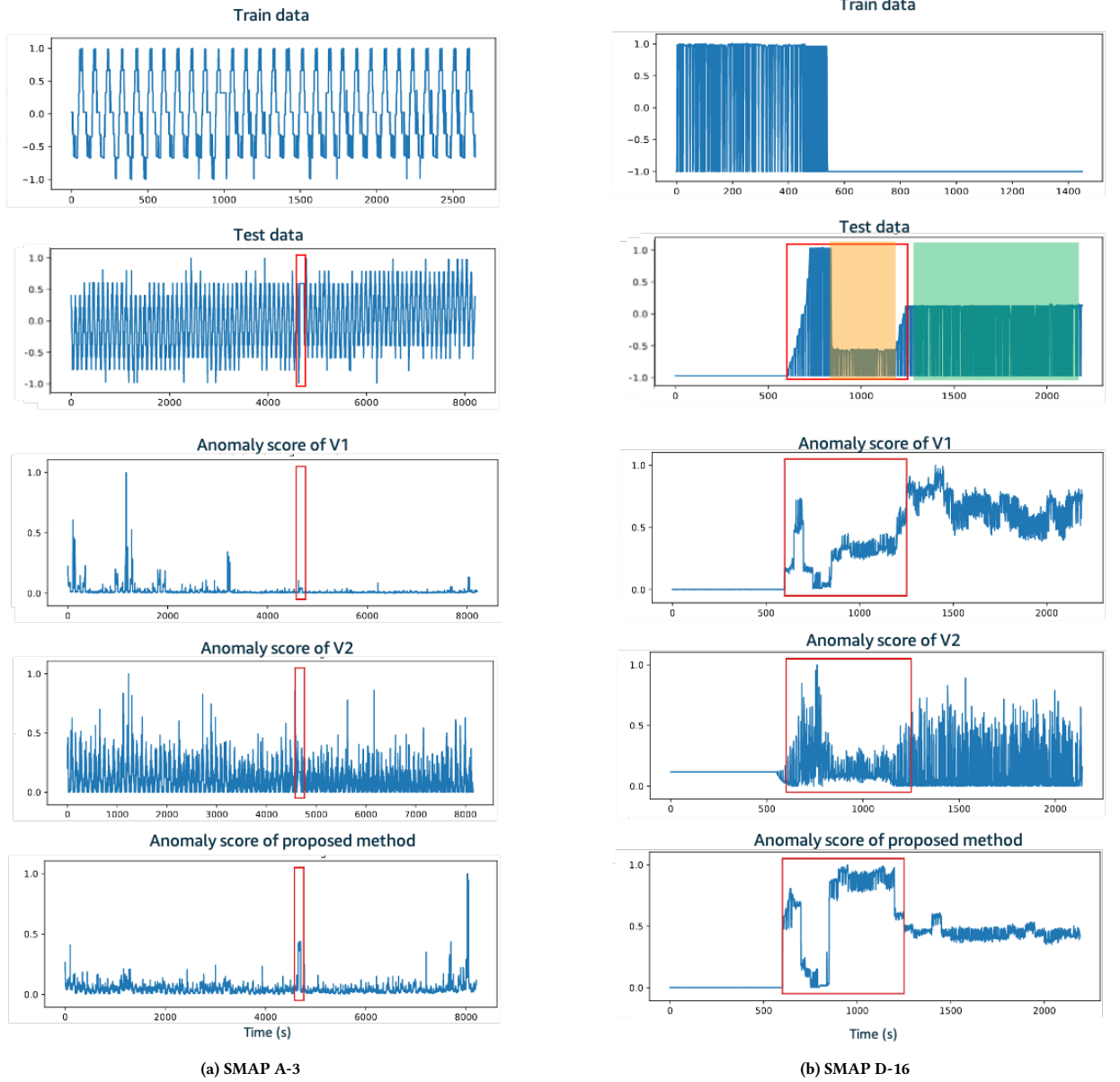
Figure 4: Case studies on SMAP dataset to show the effectiveness of proposed method.
