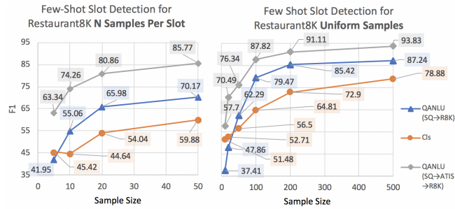
Fig. 2: Slot detection with QANLU vs token classification. SQ→R8k indicates QANLU first trained on SQuAD2.0 and the fine-tuned on samples of Restaurants-8k. SQ→ATIS→R8k is QANLU first trained on SQuAD2.0, then fine-tuned on entire ATIS, and then fine-tuned on samples of Restaurants-8k (sequential transfer learning). Cls is for the token classification approach. Numbers associated with each point are F1 scores.
