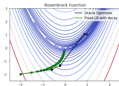
Figure 1: A toy-example of the solution to (1) using the two-dimensional Rosenbrock function (left). For the same initial condition, gradient descent with decaying learning rate of 1/t converges to a sub-optimal value. The solution of (1) reaches the global optimum [1, 1] in 4 steps.
