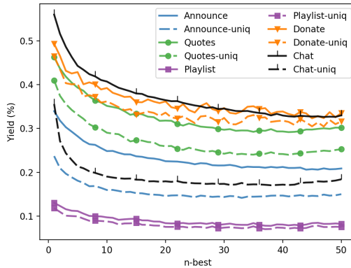
Figure 2: Validation rate for n in n -best list. Dashed line represents how many of the validated utterances are unique utterances. Paraphrases are generated by inserting bootstrap training data for each functionality.
