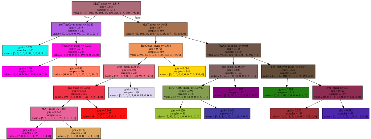
Figure 5: Final reduced decision tree after application of recursive trimming algorithm (i.e. TreeB ), resulting in 14 leaf nodes.
