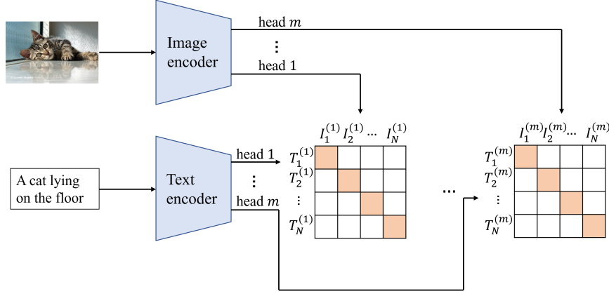
Figure 1: Our proposed multi-head CLIP method. Both image encoder and text encoder output m representations for each image-text pair ( m = 1 becomes the original CLIP model). The objective consists 3 parts as shown in (1): loss function L(\theta) , diversity regularization R_{div} and closeness regularization R_{close} .
