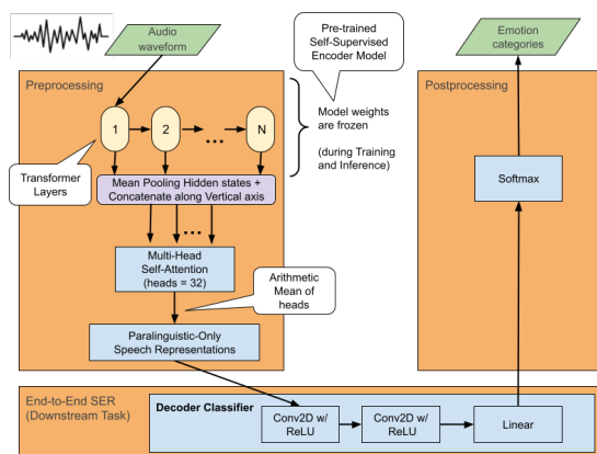
Figure 1: Proposed SER system architecture
