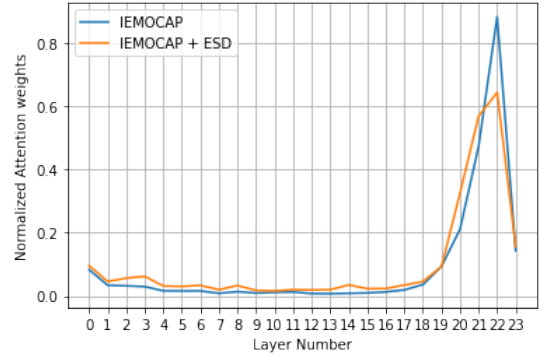
Figure 2: Layer-wise attention weights
