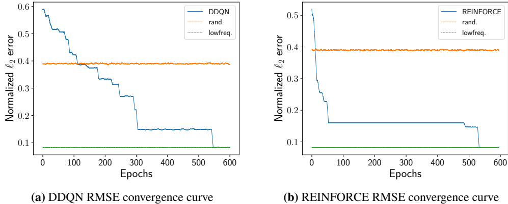
Figure 2: Convergence curve of image reconstruction error (normalized \ell_2 error) during training.
