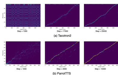
Figure 4: Evolution of attention matrix with training steps for Tacotron2 and AR-TTE
