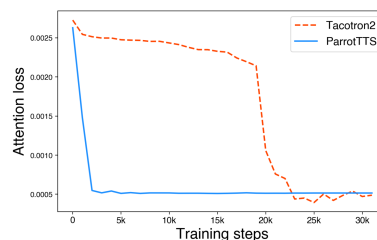
Figure 5: Attention loss plotted against training steps Tacotron2 and AR-TTE
