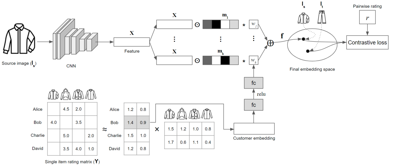
Fig. 2: PSA-Net: An overview of our proposed approach
