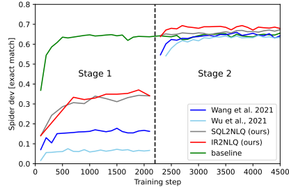
Figure 1: Comparison of different synthetic data on Spider dev set performance. The baseline model is trained using Spider data only. Previous synthetic datasets (Wu et al., 2021; Wang et al., 2021) fail to bring additional performance boost to the model. Our synthetic data (SQL2NLQ and IR2NLQ) yield better results on both stages. (Stage 1 is training with synthetic data only and Stage 2 is finetuning with real Spider training set.)
