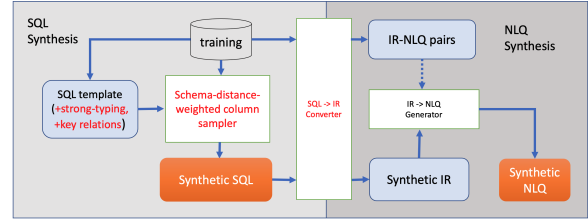
Figure 2: Our NLQ-SQL synthesis framework. Novel components include strong-typing, key relations, schema-distance-weighted column sampler, and \text{SQL} \rightarrow \text{IR} converter.
