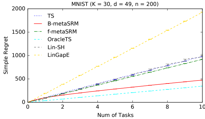
Figure 8: Cumulative average per-task simple regret for the MNIST experiment.
