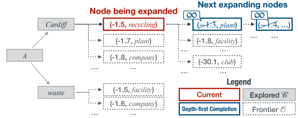
Figure 5: Depth-first completion. The red node is the current node being expanded. We depth-first expand a sequence of nodes (in blue) to get a completed path.
