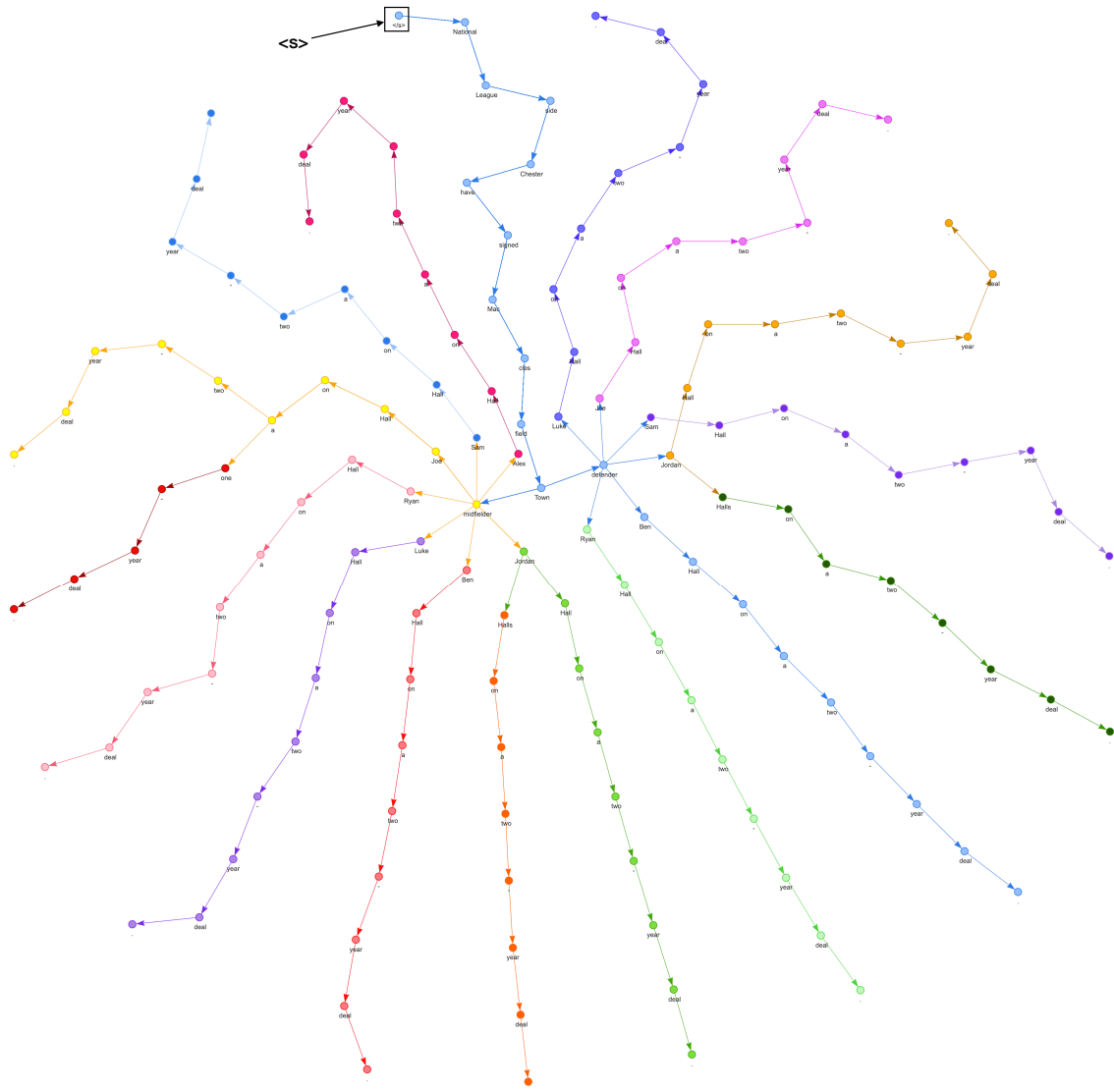
Figure 11: Visualization of one example output for beam search on XSum. n_{\text{SOS}} is labeled. Each color represents one unique ending.
